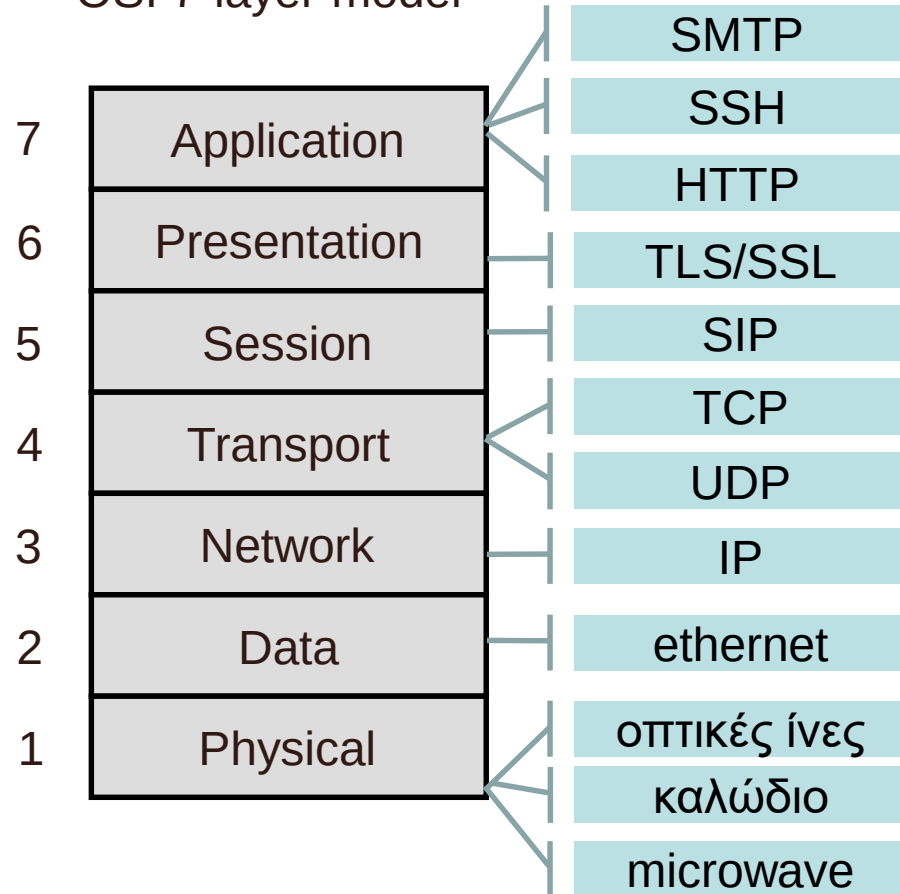
OSI 7-layer model
