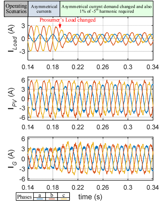
Fig. 9: Experimental results validating the significance of proposed innovative control scheme for effective mitigation of prosumers abnormalities.
